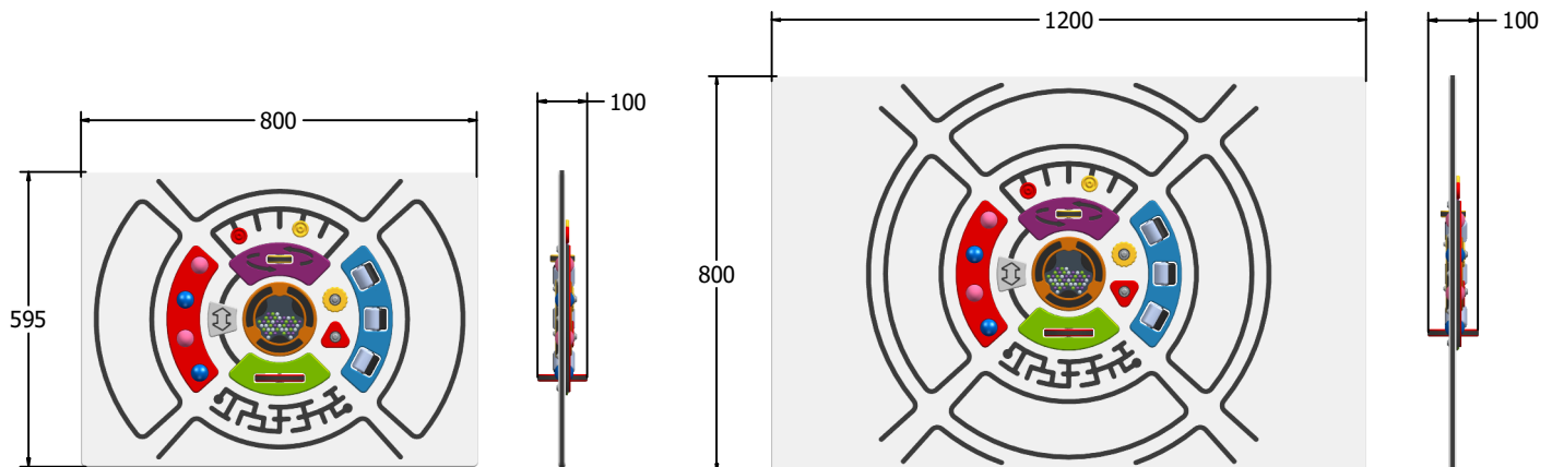
FISENFID3 Standard Panel FISENFID3-AL-WP Panel with Alu Posts
