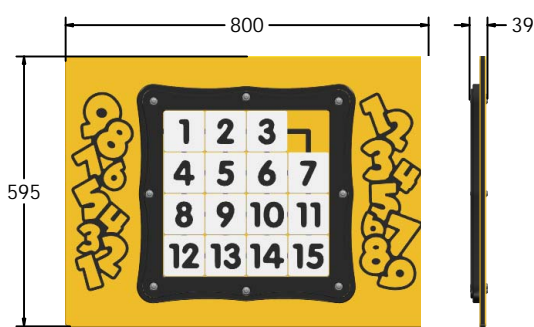
FITSNUM6 Standard Panel FITSNUM6-AL-WP Panel with Alu Posts
