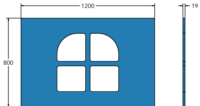
FIWINDOW3 FIWINDOW3 -AL-WP Standard Panel Panel with Alu Posts
