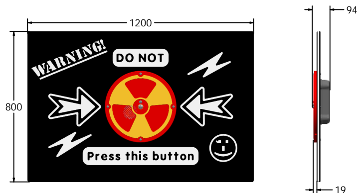
FIPTDONOT3 Standard Panel FIPTDONOT3-AL-WP Panel with Posts
